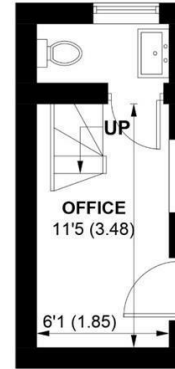
OUTBUILDING - GROUND FLOOR
